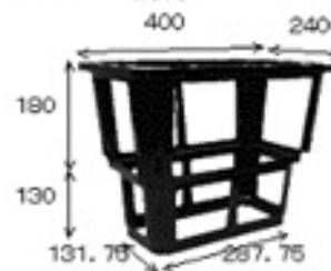
CF-401 (付屬)
